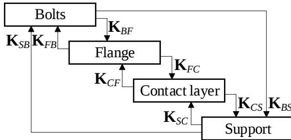
FIG. 2. Feedback loops between the subsystems of the multi-bolted system.
