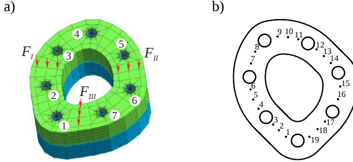
FIG. 3. Model of the system: a) FEM-based model, b) nodes adopted to describe the normal contact pressure distribution ( F_I = F_{II} = F_{III} = 30 kN).
