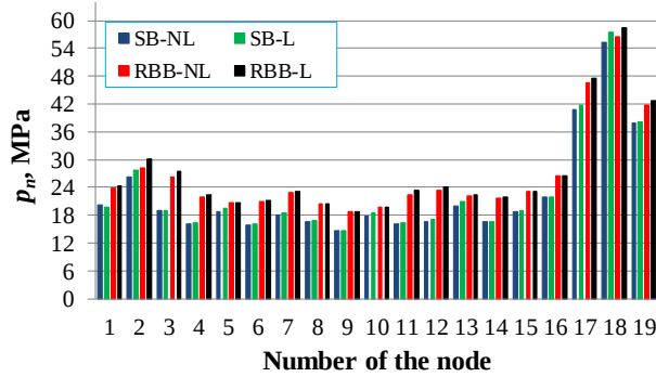
FIG. 4. Distributions of normal contact pressure at the interface of the joined parts for the model loaded by: a) F_I , b) F_{II} , c) F_{III} .
