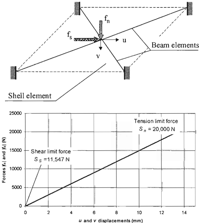
FIG. 4. Model of the bolted connection. Top: a grid of four beam elements connecting a spotweld on the post with four nodes on the W beam. Bottom: shear and tension force–displacement characteristics assumed for FE models of bolts.
