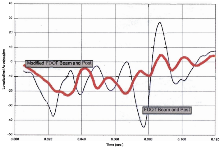
FIG. 14. Acceleration histories for the original and the modified Florida Beam-and-Post bridge barrier, simulations 6-3 and 6-4. Note: longitudinal accelerations (vertical axis) are provided in terms of earth acceleration g . Data averaged over 10 milliseconds.
