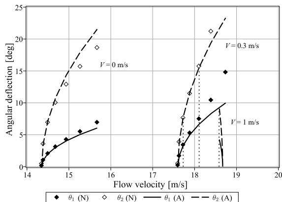
FIG. 2. Bifurcation diagram of the intermediate propulsor for swimming speeds V = 0 m/s, 0.3 m/s, 1 m/s, lines – analytical approximation of amplitude \theta_1 (solid) and \theta_2 (dashed), diamonds – amplitude values obtained numerically.
