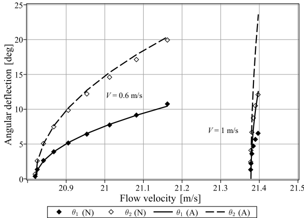
FIG. 8. Bifurcation diagram of the high-speed propulsor at swimming speeds V = 0.6 m/s and V = 1 m/s, lines – analytical approximation of amplitude \theta_1 (solid) and \theta_2 (dashed), diamonds – values obtained numerically.
