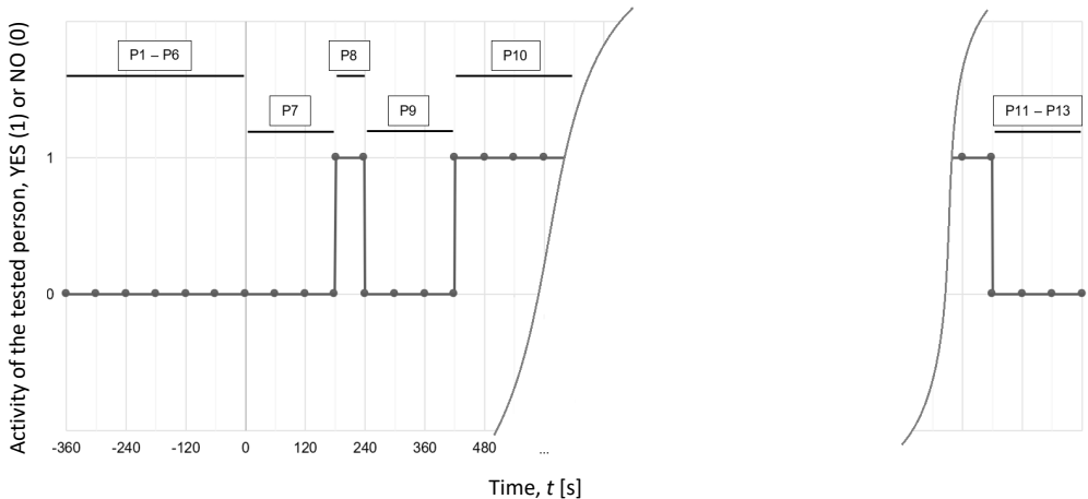
FIG. 5. Schematic diagram of the test procedure aimed at developing the power graph.
