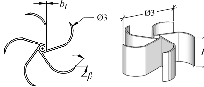
FIG. 3. Dimension and outline of the blade.
