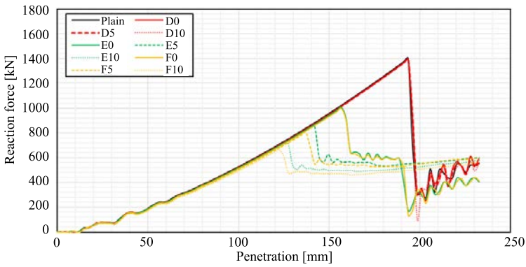
FIG. 13. Reaction force in the grounding simulation for the plain plate, scenarios D, E, and F.
