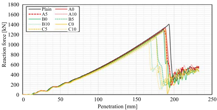
FIG. 12. Comparison of the reaction force in all grounding simulation scenarios.
