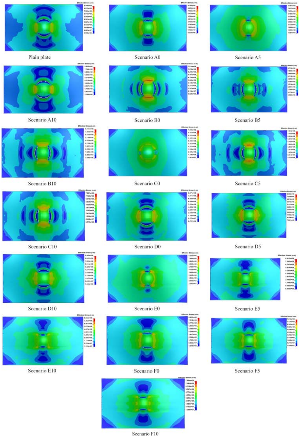
FIG. 16. Crack initiation at all grounding scenarios.
