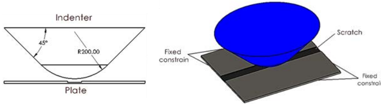
FIG. 9. Boundary condition of grounding simulation.
