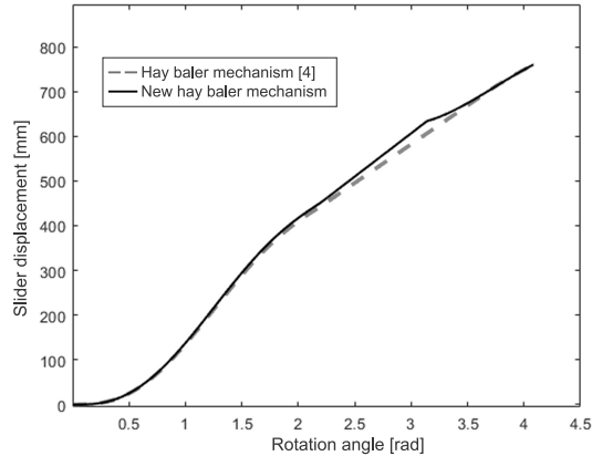
FIG. 11. Displacement comparison chart.
