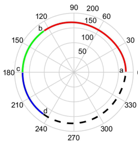
FIG. 7. Pitch curve for the driven non-circular gear.
