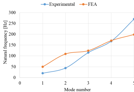
FIG. 22. Comparison of experimental values with FEA for 0% CFF.
