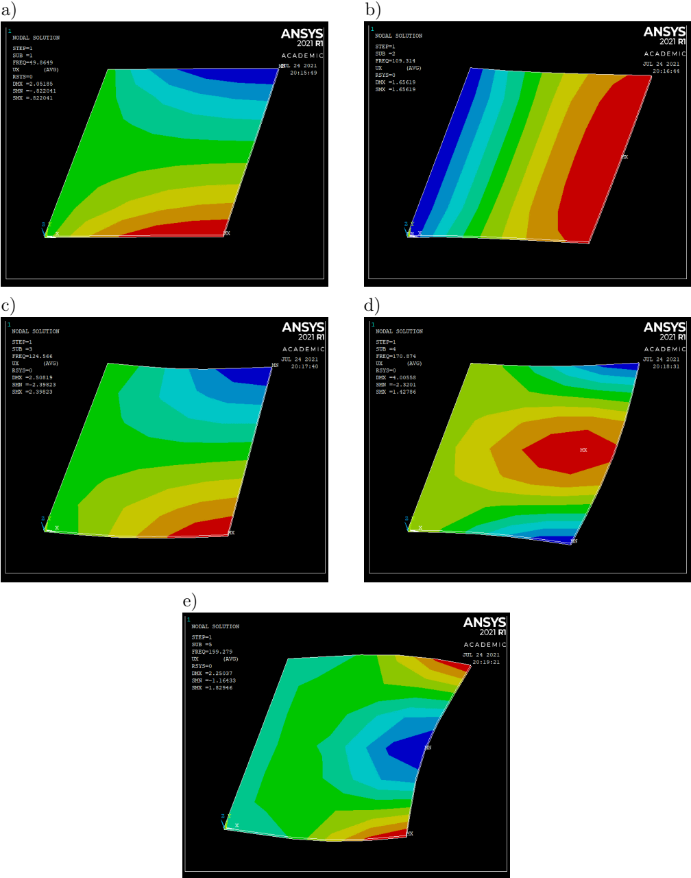
FIG. 18. FEA mode shapes for 0% CFF composite specimen.
