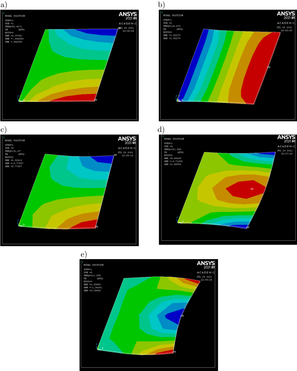
FIG. 20. FEA mode shapes for 20% CFF composite specimen.
