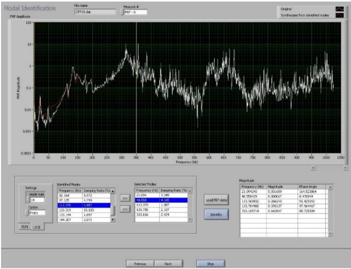
FIG. 10. Magnitude–frequency response-10% CFF content composite.
