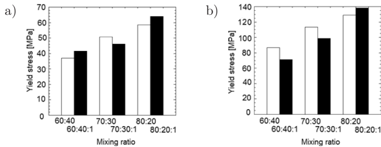
FIG. 7. Effect of the PBAT content on the compression yield stress at a) low strain rate and b) high strain rate.
