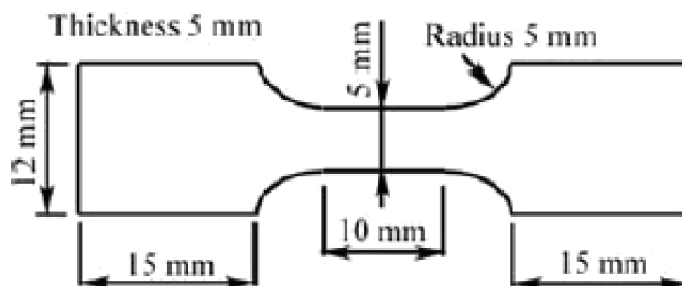
FIG. 1. Specimens for the quasi-static tension test, used in the case of the cornpole CPR-M2.
