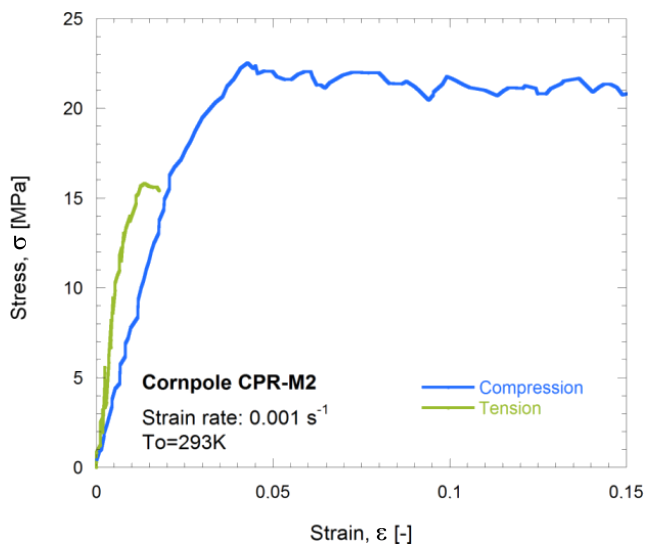
FIG. 3. CPR-M2. Results of the tension and compression tests.
