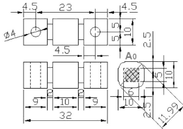
FIG. 2. Geometry of the specimen for the double shear test, the shear zone is indicated by gray shading.
