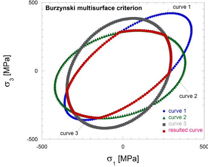
FIG. 8. Representation of the elastic domain based on Burzyński multi-surface criterion in the plane \sigma_2 = 2 , the resultant limit curve is expressed by the red line.
