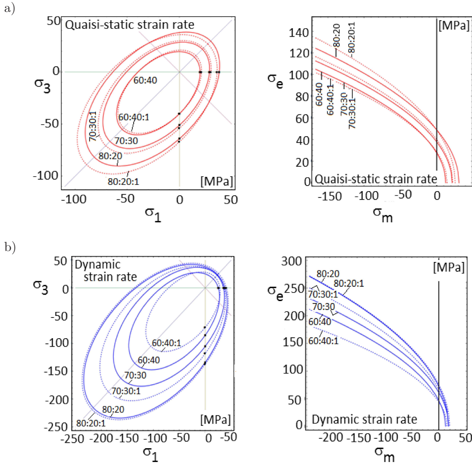
FIG. 10. Yield curves in the plane \sigma_2 = 0 and meridional plane for polymers with different proportions of PLA/PBAT at: a) quasi-static strain rate, b) dynamic strain rate. Polymers with addition of dialkyl peroxide are indicated by dotted curves.
