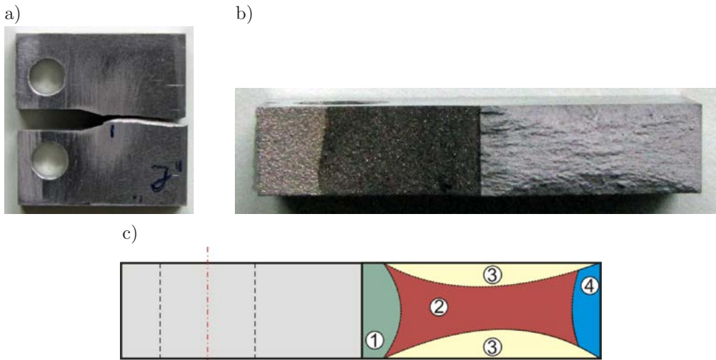
FIG. 12. Specimen made of the 44200+20% Saffil fibre composite after tests for K IC : a) specimen, b) entire fracture surface, c) fracture surface scheme: 1 – fatigue area, 2 – fracture zone, 3 – sloping fracture surfaces, and 4 – tearing zone.
